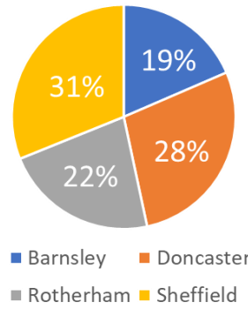
Figure 3 Emissions split by sub-region
